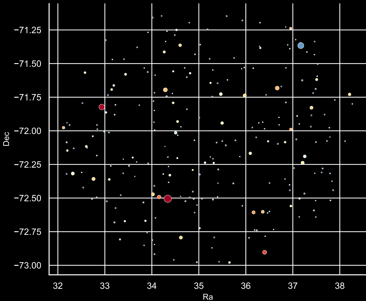
Field [95] Ra [35.19] Dec [-72.05] Stars: 236
