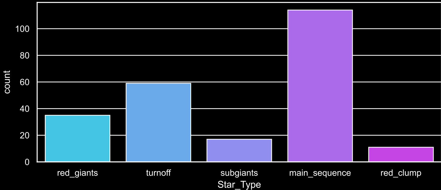
Field [95] Count plot of Star Type
