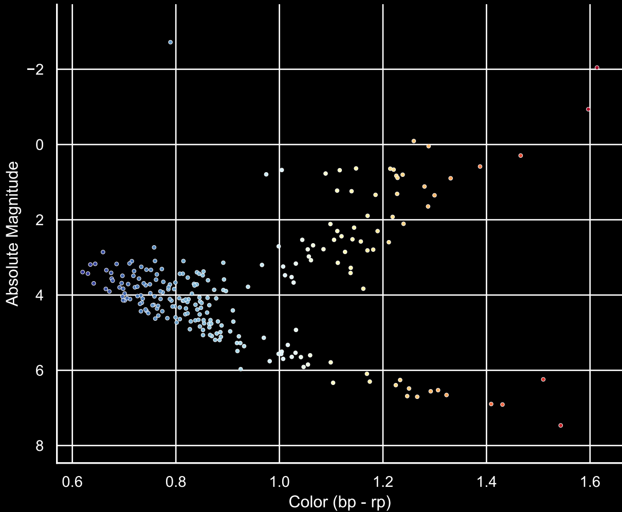
GALAH Hertzprung-Russel Diagram Field [95] Ra [35.19] Dec [-72.05]
