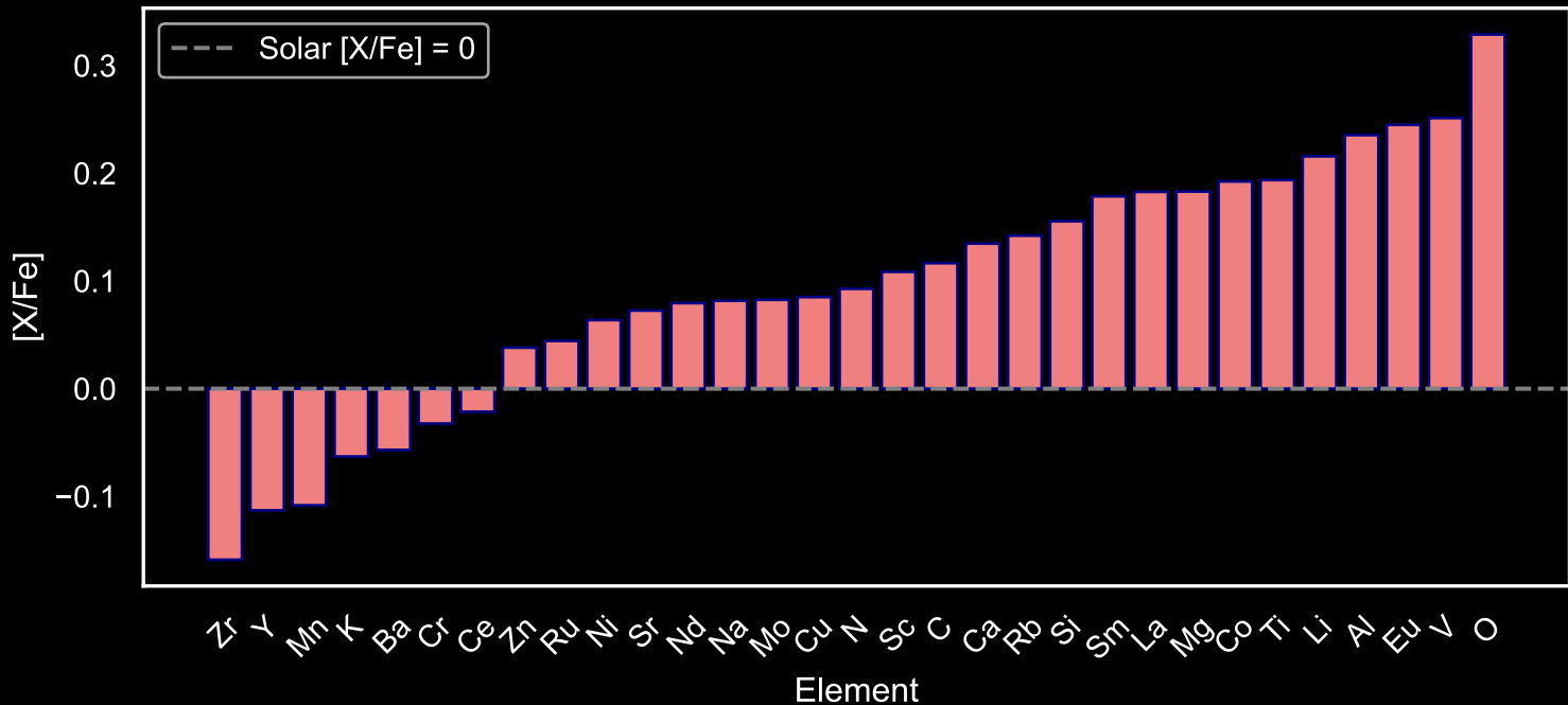
Abundance Pattern for GALAH Red Giants: Star Field [95] (N=46)
