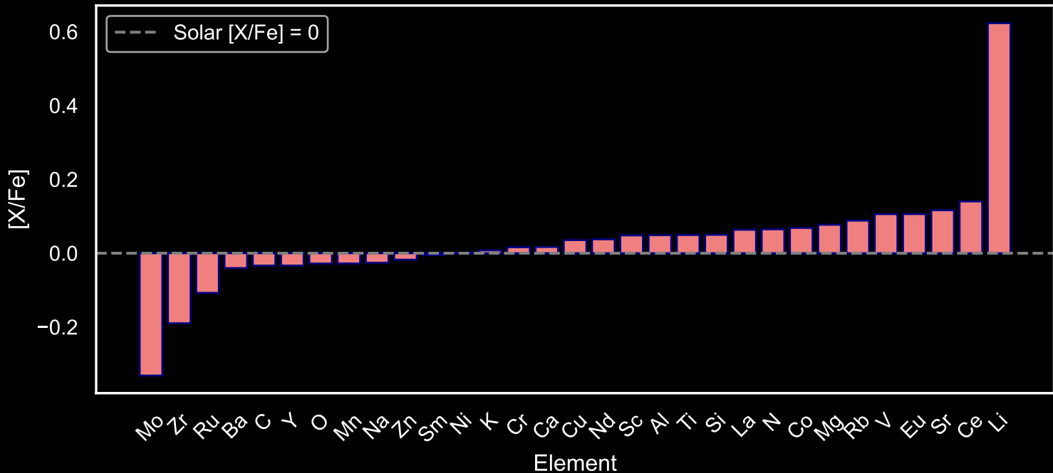
Abundance Pattern for GALAH Main Sequence Stars: Star Field [95] (N=114)
