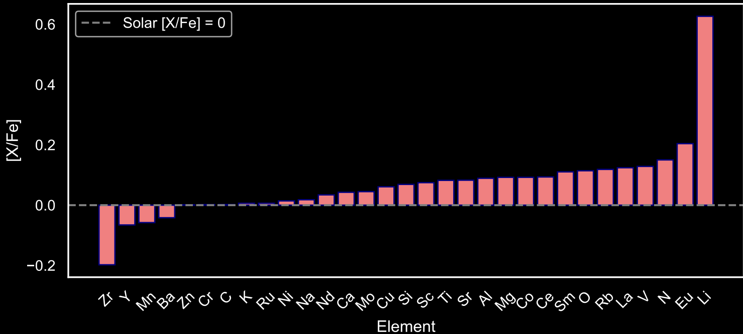
Abundance Pattern for GALAH Star Field [95] (N=236)
